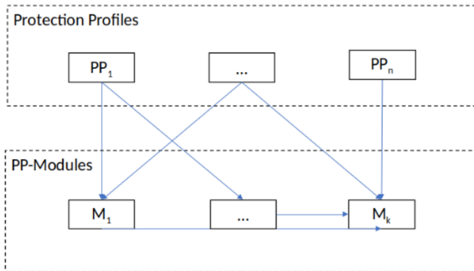
Representation of a PP-Configuration composed of PP_1 \dots PP_n and M_1 \dots M_k , where n \geq 2 or k \geq 1
